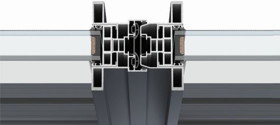
FINISHING TREATMENT OF CORNER DOORS
