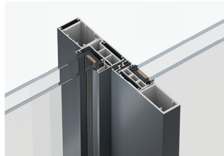
32MM REINFORCED HOOK (FIXED WINDOW)
